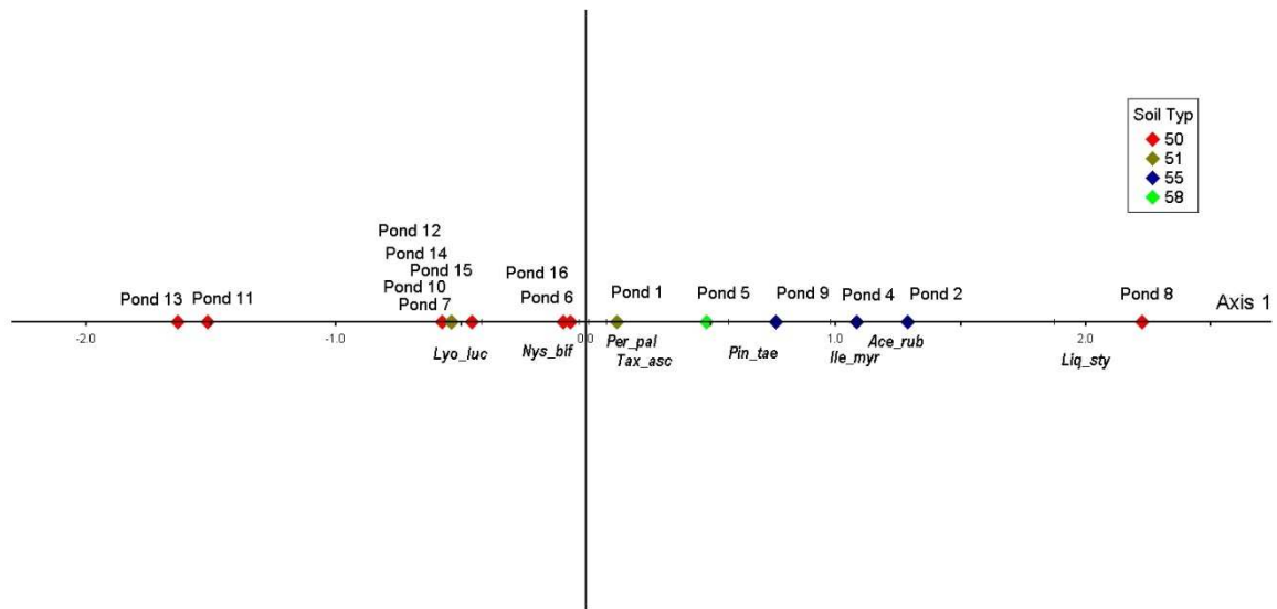
Figure 2.3: NMS Axis 1 ordination of wade ponds. Legend displays the soil ID numbers with assigned color coordination.
